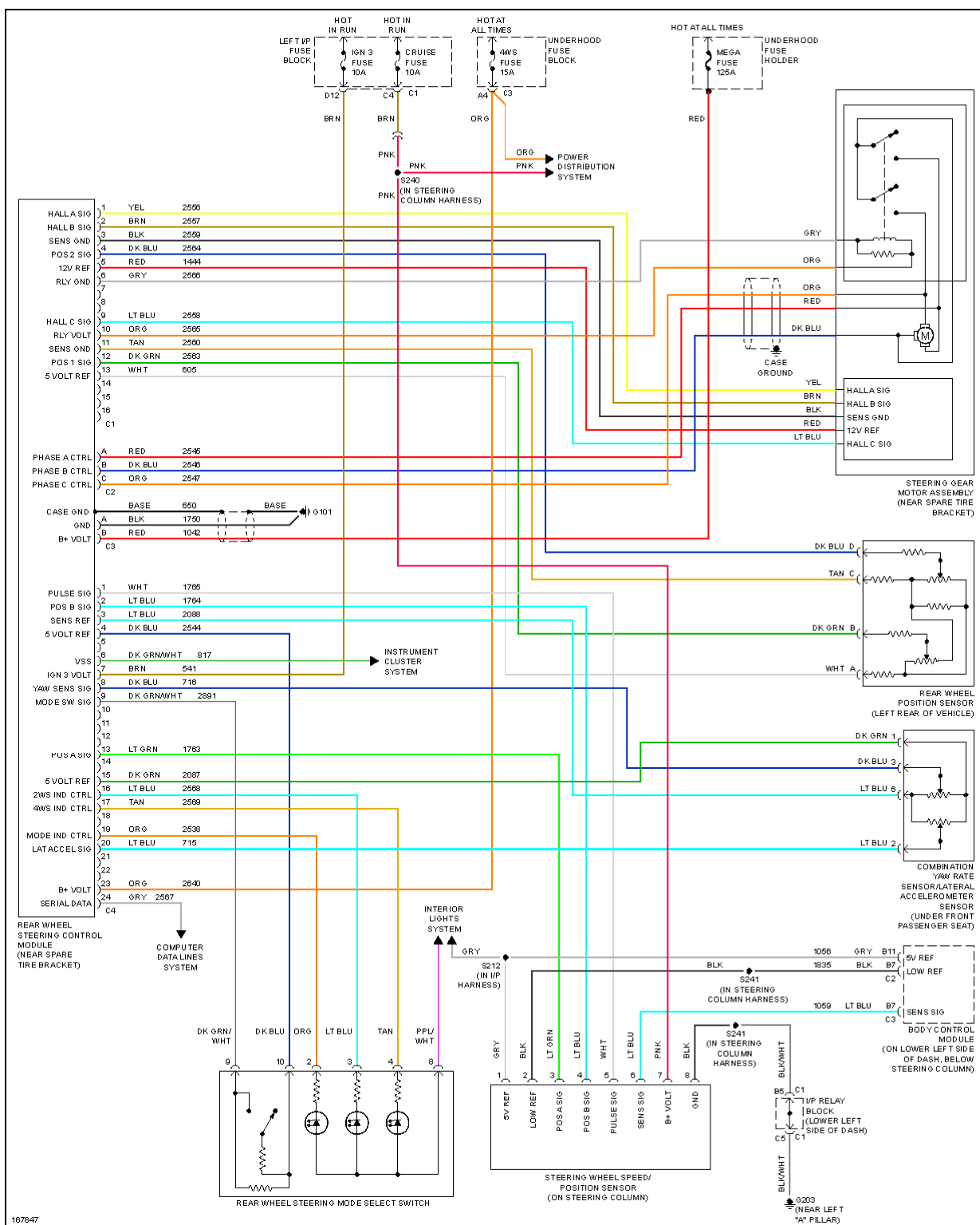
Fig. 21: Rear Wheel Steering Circuit
